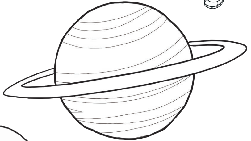
Saturn
